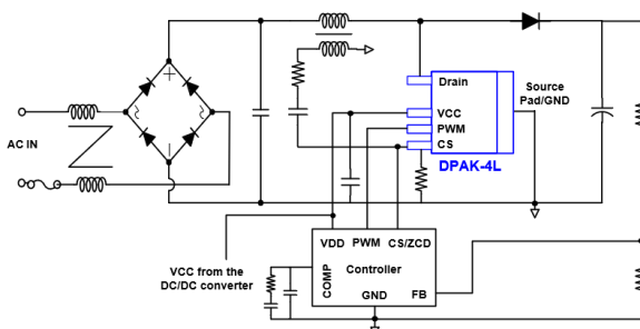
Boost PFC
