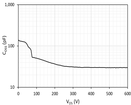
Figure 9. Output capacitance ( C_{OSS} ) vs. drain-to-source voltage ( V_{DS} )
