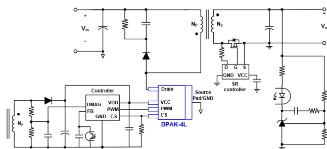
QR Flyback
