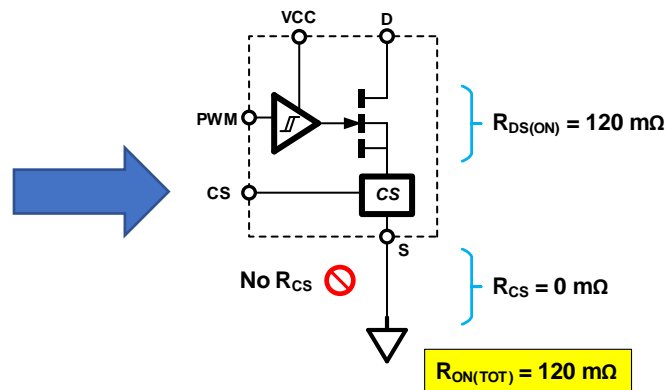
Figure 23. External resistor sensing vs. GaNSense™ Technology
