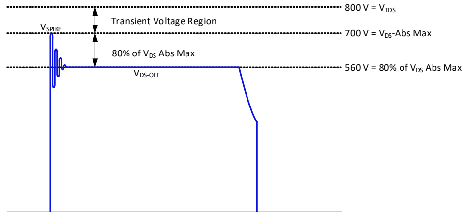
Fig. 29. QR flyback drain-to-source voltage stress diagram
