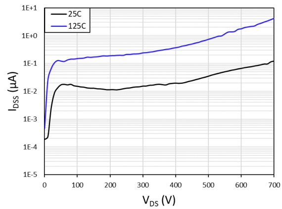
Fig. 5. Drain-to-source leakage current ( I_{DSS} ) vs. drain-to-source voltage ( V_{DS} ) at T = 25\text{ }^{\circ}\text{C} and T = 125\text{ }^{\circ}\text{C}
