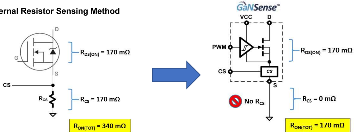
Fig. 26. External resistor sensing vs. GaNSense™ Technology
