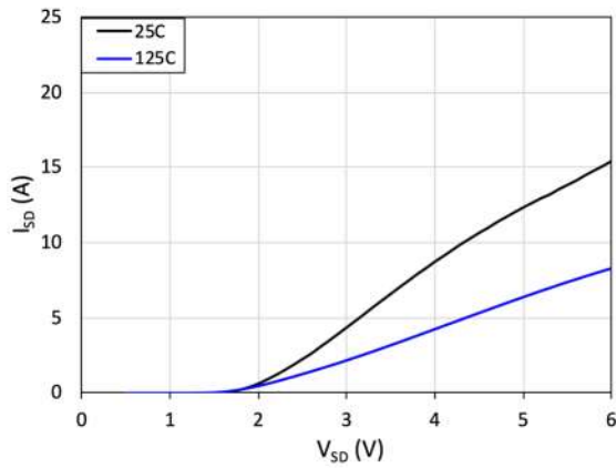
Fig. 4. Source-to-drain reverse conduction voltage vs. source-to-drain current ( I_{SD} ) at T = 25\text{ }^{\circ}\text{C} and T = 125\text{ }^{\circ}\text{C}
