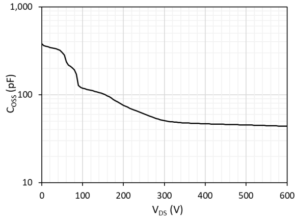
Fig. 9. Output capacitance ( C_{OSS} ) vs. drain-to-source voltage ( V_{DS} )
